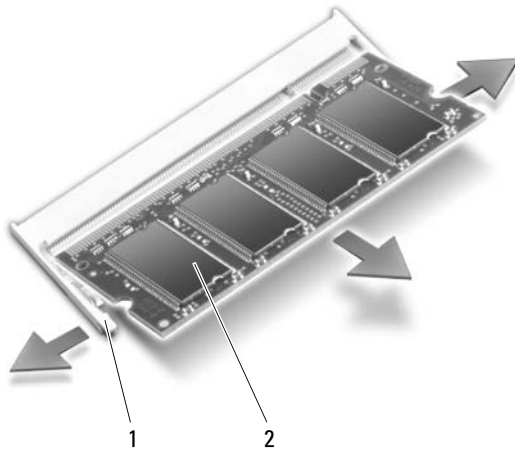
1 securing clips (2) 2 memory module (DIMM 1)
